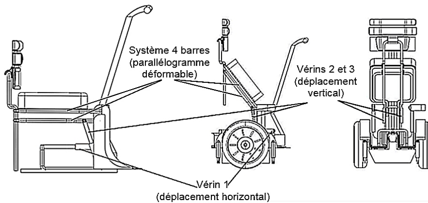
figure 4 - Principe de verticalisation.
